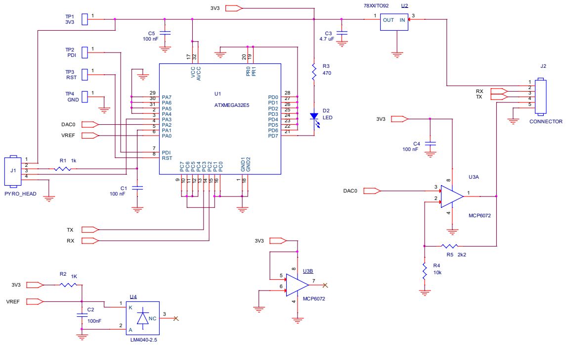
Fig.2. Digital Board Schematics.
