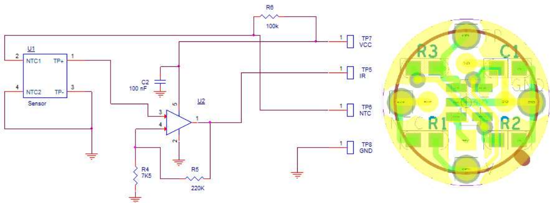
Fig.3. Pyro Head Electronics.
