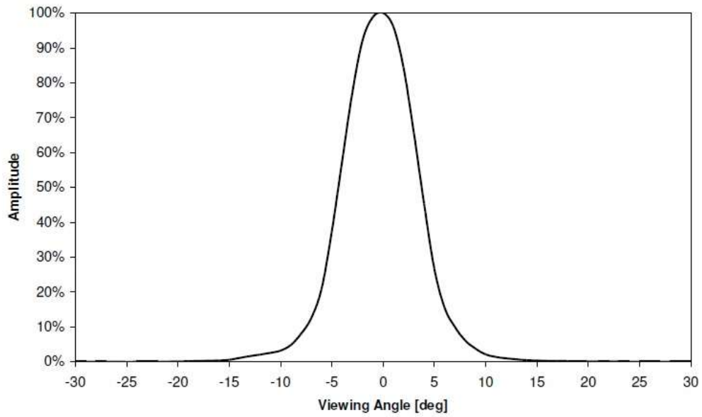
Fig.4. Optical Lens viewing angle-
